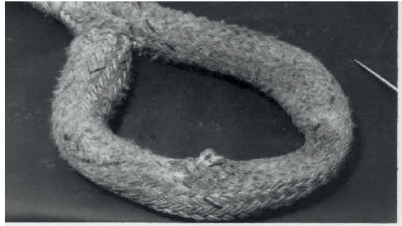
Figure no. 11 b): damage of splicing - wear in double braid eye splice
