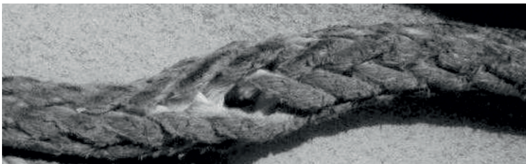
Figure no. 4: Inter-strand abrasion (exposed internal area reveals wear at strand internal contact points)
