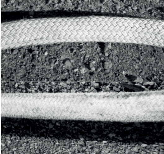
Figure no. 2: Fibre abrasion - Cyclic tension
