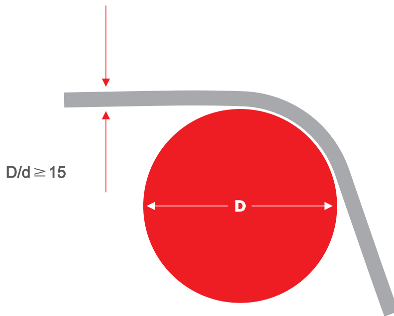
Figure no. 10: D/d ratio of mooring line to deck equipment
